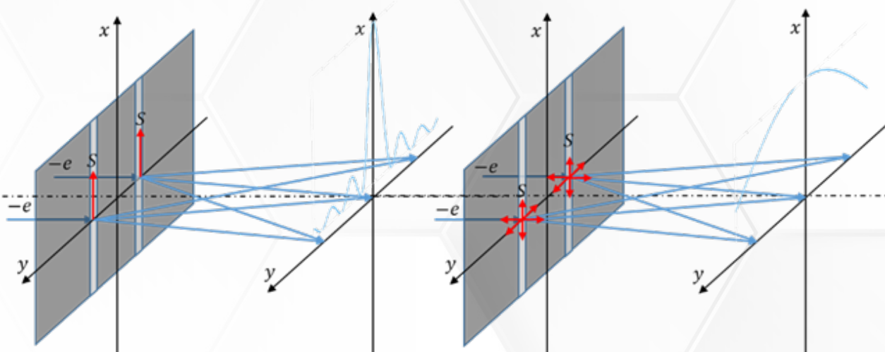
Fig.4 Electron Interference. (a) With the same spin state (tensor potential A^\mu ).(b) Spin state (tensor potential A^\mu ) is changed by any reason, such as ‘observation’.
