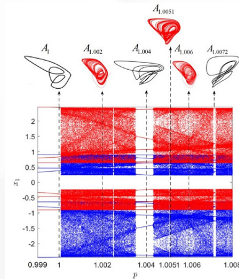
Fig.1 . Bifurcation of the HNN system for p \in [0.999, 1.008] of the component x_1 , after transients are removed. Several chosen parameters with their corresponding attractors are indicated.
